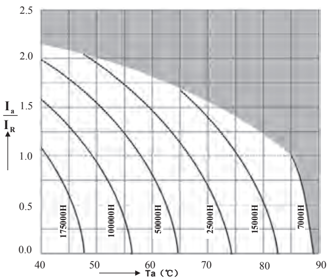
depending on ambient temperature T a versus under ripple current operating conditions VR ≤ 100V
