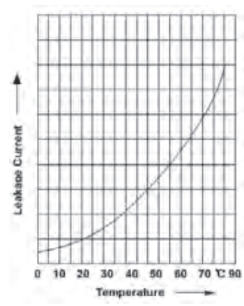
Figure 12 Temperature vs Leakage Current
