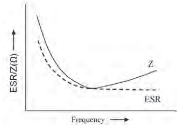
Figure 10 Impedance vs ESR vs Frequency
