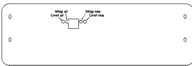
ADC7480 front panel Location of tuning trimmers for analog control Trimmers are covered by sticker
