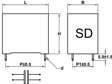
4 terminals execution
