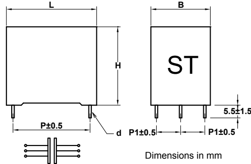
6 terminals execution
